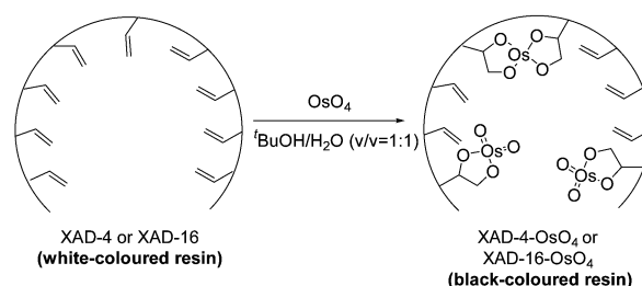
Fig. 1 Osmylated macroporous resins.
